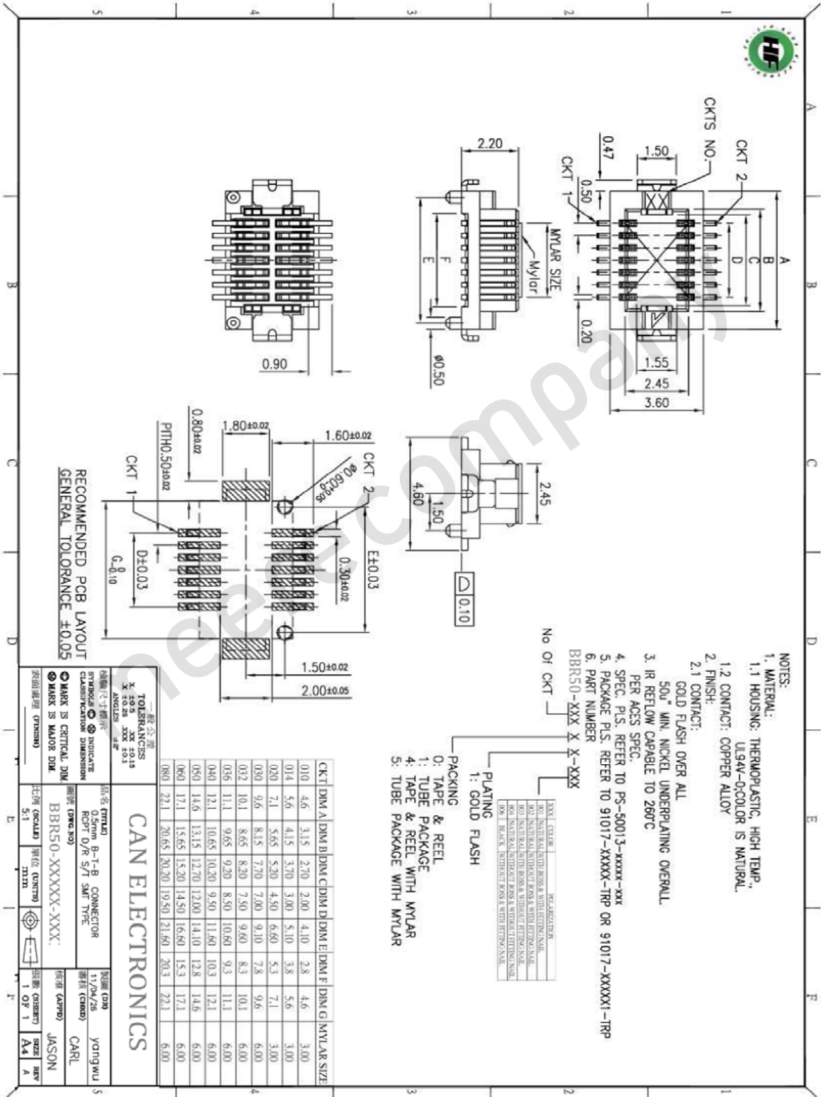
Fig 14. S100D connector
